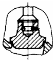
regulation disc
