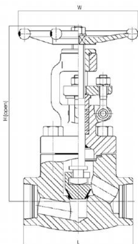
Threaded ends
