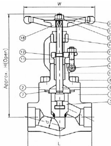
Socket welding ends
